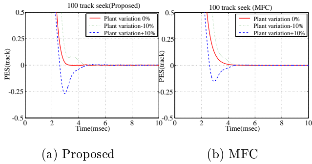
Figure 10: 100 track seek (simulation)
