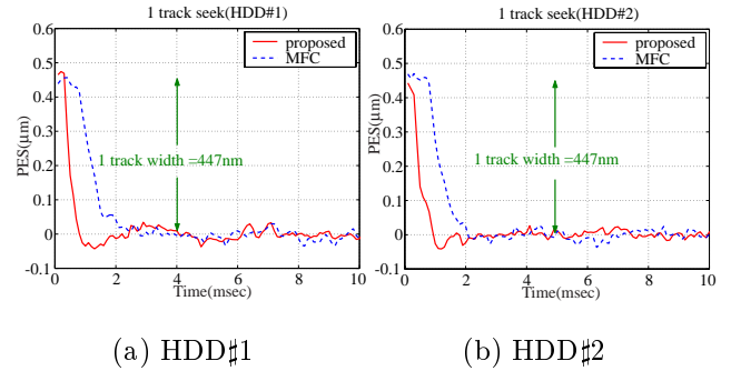
Figure 12: 1 track seek (experiment)
