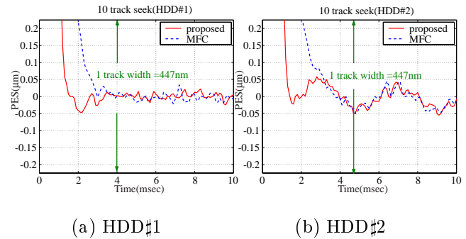
Figure 13: 10 track seek (experiment)
