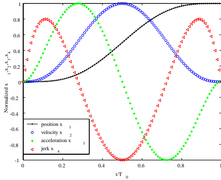
Figure 3: Normalized trajectory based on the equation (15) ~ (18)
