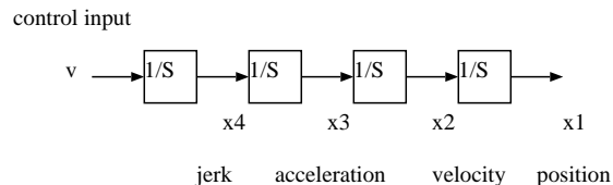
Figure 1: Simple model of VCM
