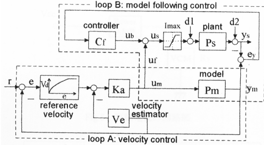
Figure 5: Model Following Control system
