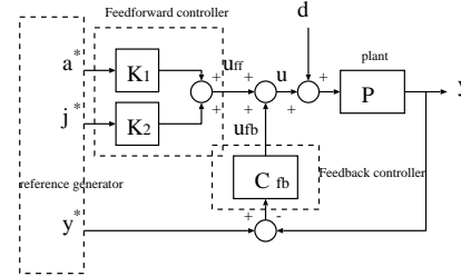
Figure 7: Reconstructed positioning control system
