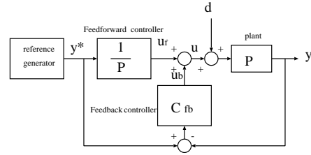
Figure 6: Ideal block diagram
