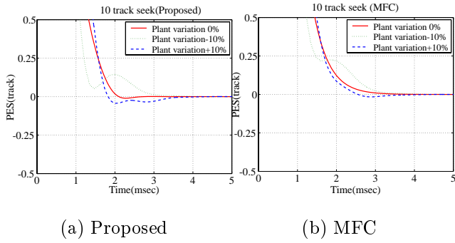
Figure 9: 10 track seek (simulation)
