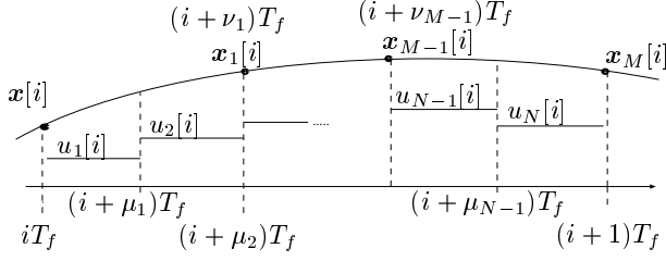
Fig.3: Multirate sampling control.
