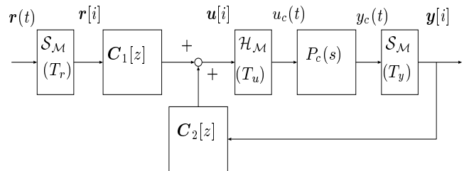
Fig.2: Two-degree-of-freedom control system.
