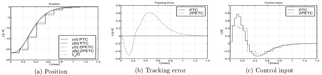
Fig.9: Simulation results B (6trk).
