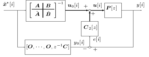
Fig.6: Structure of the proposed controller.
