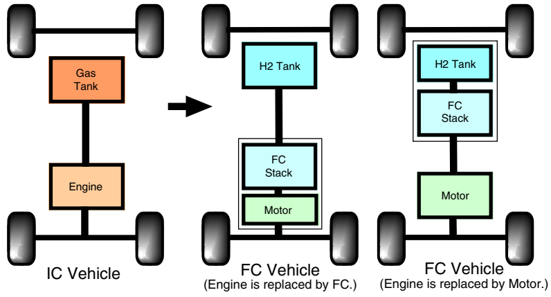
Fig. 29. Two ways to understand FCV.
