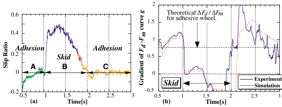
Fig. 23. Experimental results of wheel skid detector.
