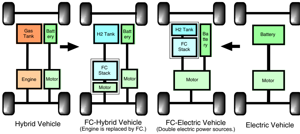
Fig. 30. Two ways to understand FCV with battery, FCHV or FCEV?
