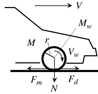
Fig. 8. One wheel model.
