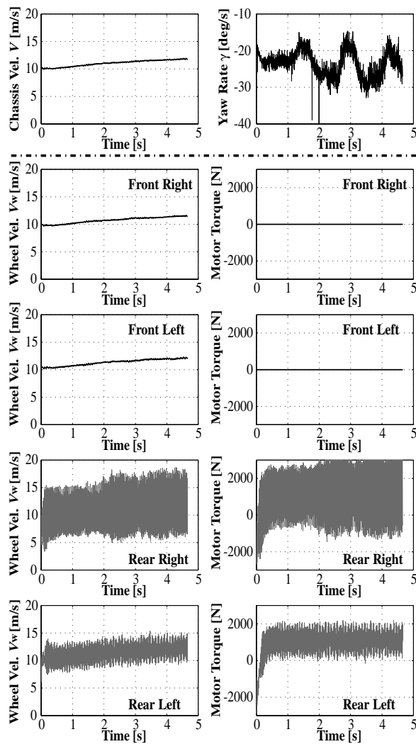
Fig. 19. Vehicle stabilizing effect of our proposed controller MFC.
