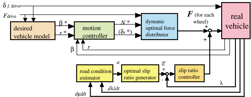
Fig. 28. Implementation of SRC into the whole control system.
