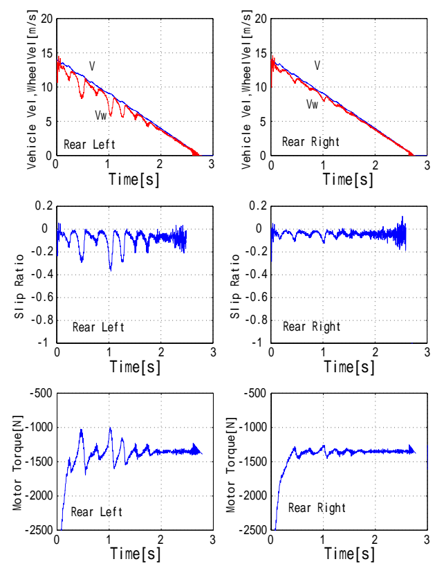
Fig. 11. Stable braking with our proposed controller “MFC”.
