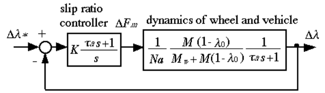
Fig. 15. Slip ratio controller (SRC).
