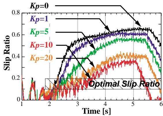
Fig. 12. Experimental results of MFC for skid prevention with \tau = 0.1 .
