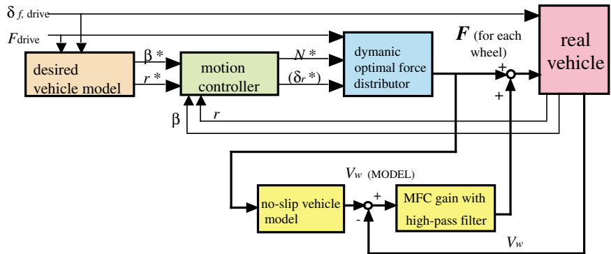
Fig. 27. Implementation of MFC into the whole control system.
