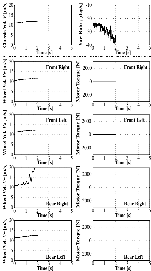
Fig. 18. Unstable cornering with sudden acceleration without MFC.
