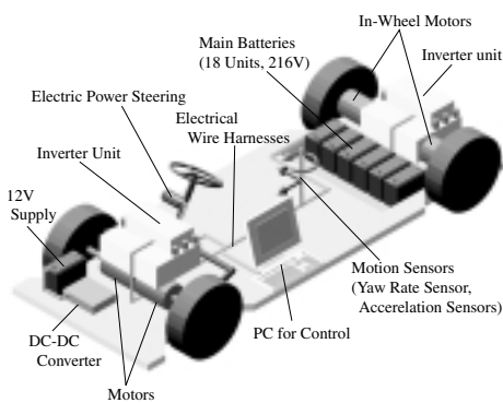
Fig. 1. Sketch to of “UOT March II”.
