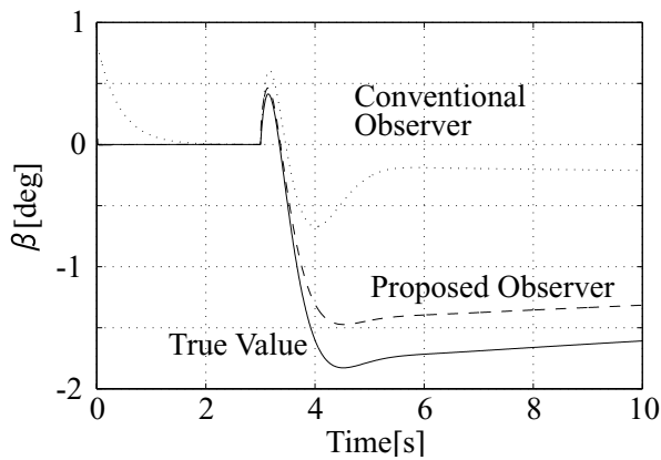
Fig. 25. \beta estimation using linear observer based on \gamma and a_y signals.
