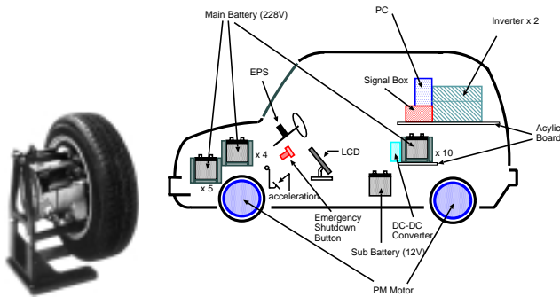
Fig. 3. In-wheel motor / Configuration of “UOT Electric March II”.
