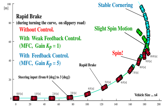
Fig. 17. Stabilizing effect with controlled four wheels is visualized with vehicle trajectory.
