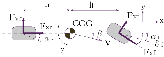
Fig. 24. Two wheel vehicle model.
