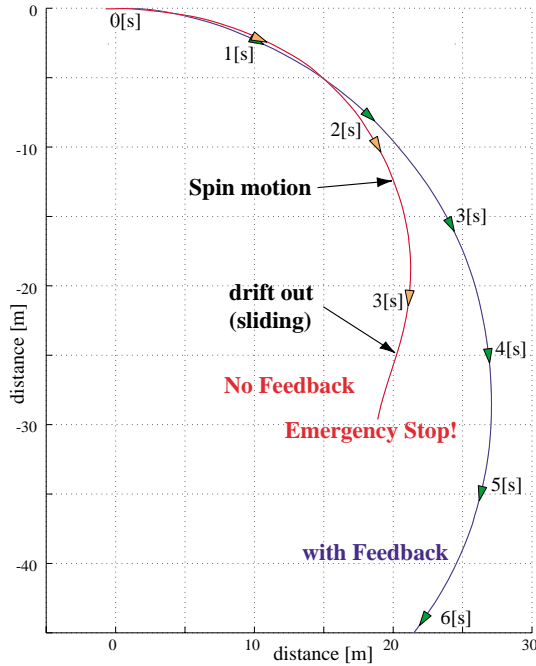
Fig. 21. Stabilizing effect of MFC installed in each wheel.
