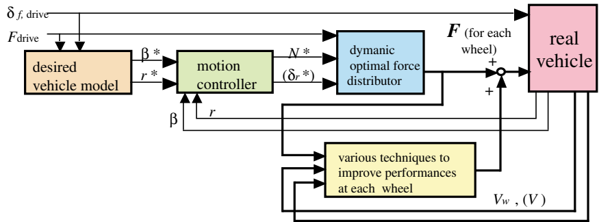
Fig. 26. Whole schematic diagram of the total control system.
