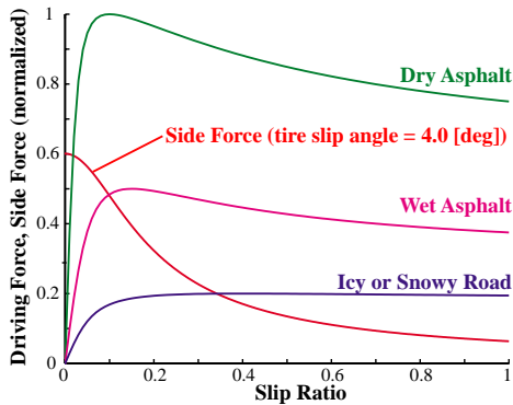
Fig. 14. Typical \mu - \lambda curve.
