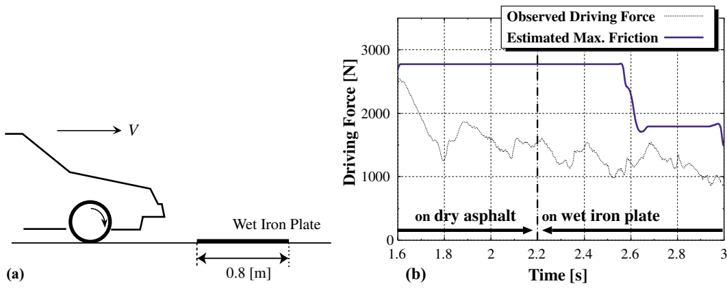
Fig. 22. Experimental results of road condition estimator. The sudden road condition change (a) was sensed with estimated maximum friction force as shown in (b).
