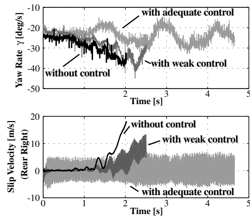
Fig. 20. Comparison of vehicle motion observed in \gamma and the slip velocity.
