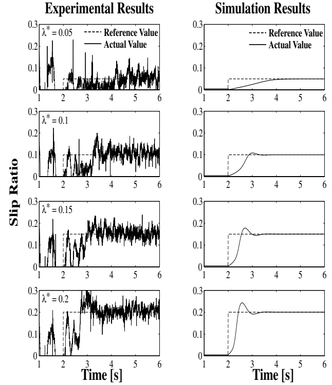
Fig. 15. Slip ratio controller (SRC).
