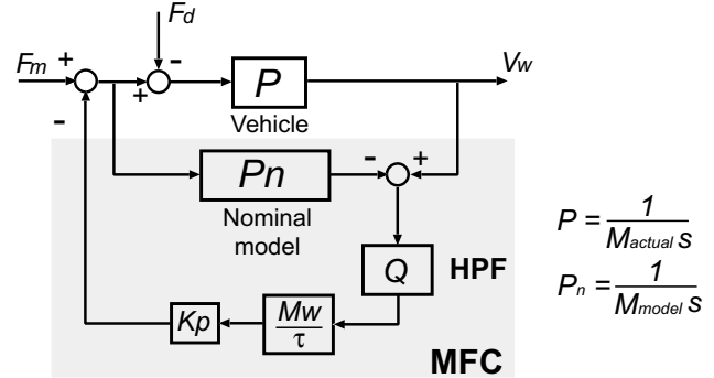
Fig. 9. Block diagram of the proposed feedback controller "MFC".
