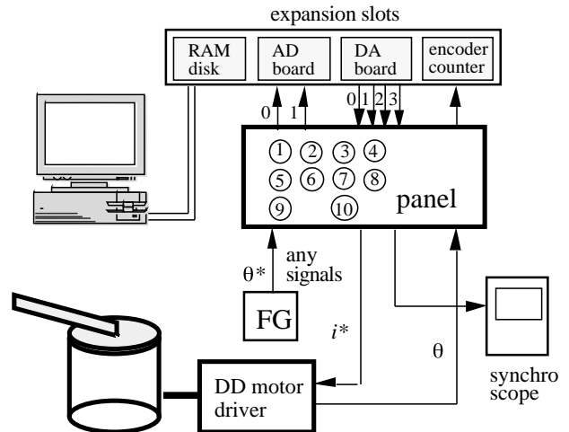
Fig. 1 Student experiment of Servo Control for all 3rd year students in undergraduate course.
