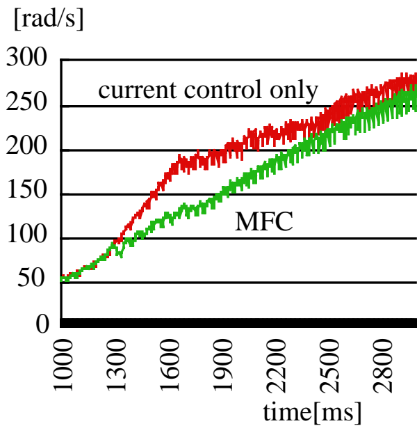
(c) wheel speed
