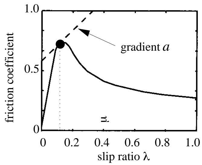
Fig.8. Nominal slip ratio is given by a=1 .
