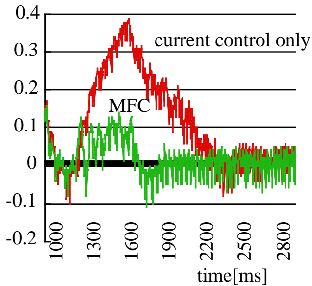
(b) slip ratio
