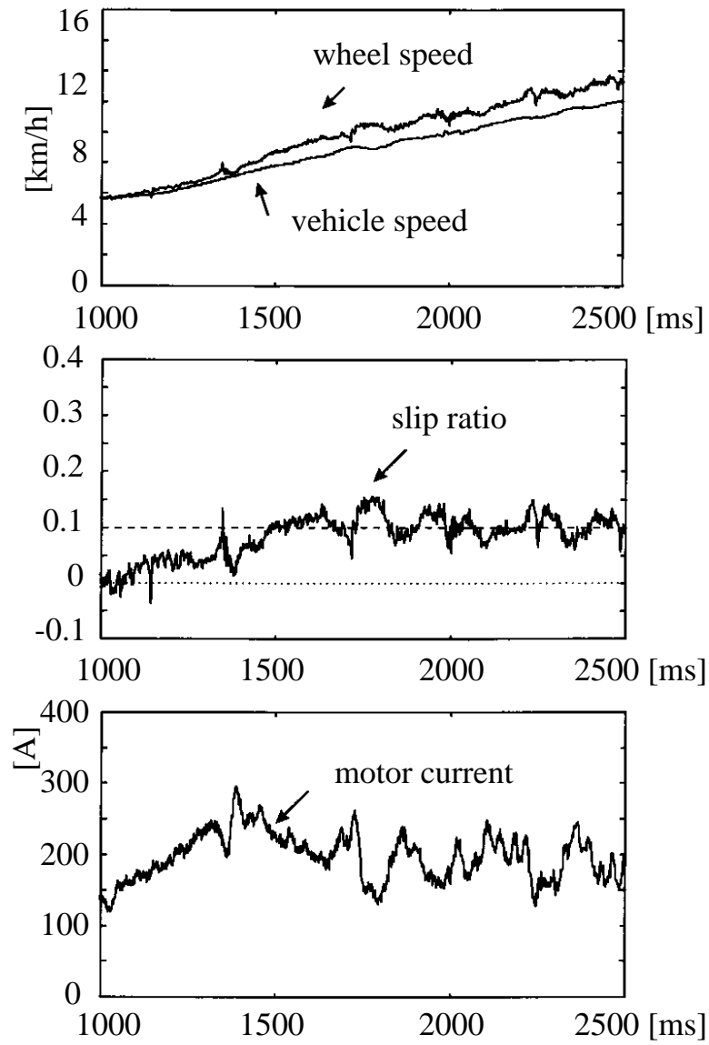
(a) constant slip ratio command
