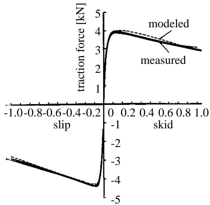
Fig.11. \mu - \lambda characteristics used in the simulation.
