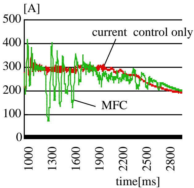
(a) motor current
