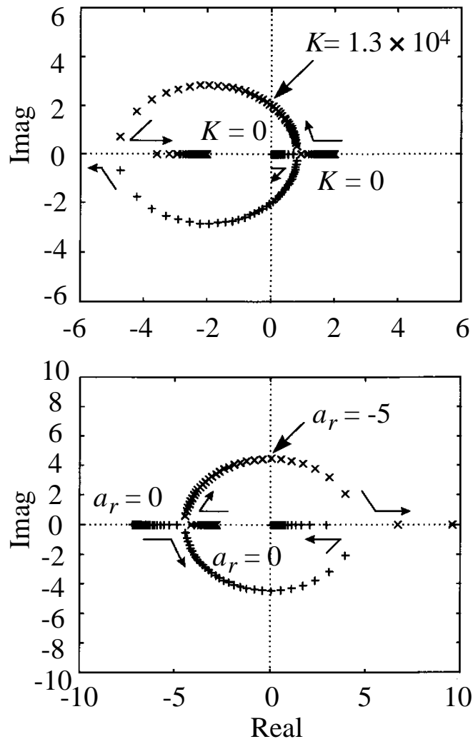
Fig.9. Root locus against parameter variation.
