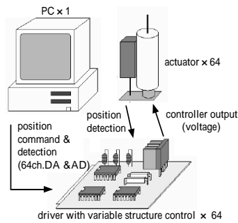
Fig. 2. Fundamental conceptual figure of experimental setup consisting of 64 variable structure controllers, 64 linear drive actuators and "one" PC.
