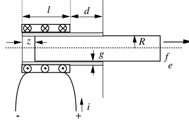
Fig. 7. Electromagnetic model of the solenoid plunger. Electromagnetic force generated in this solenoid plunger is calculated by using this simple model.
