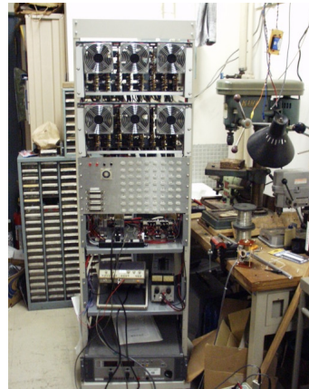
Fig. 3. Overview of experimental setup including 64 controllers and main power supply.
