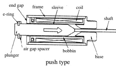
Fig. 6. Configuration of the solenoid plunger.
