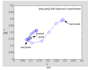
Fig. 15-b. Ping-pong ball trajectory (experiment).
