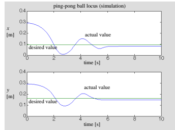
Fig. 12. Ping-pong ball locus (simulation). Upper figure is time response of ball position along x-direction. Lower one is about y-direction. The ball converges to the desired position with vibration.
