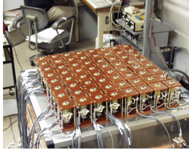
Fig. 4. A part of experimental setup, arrayed many actuators on 2-dimensional plane
