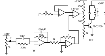
Fig. 9. Analog circuit of a variable structure controller. This variable structure controller actually used in the experiment. 64 sets of this analog circuit are prepared for realization of magic carpet. This circuit is very simple and adopted for position controller.
