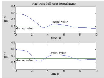
Fig. 15-a. Ping-pong ball locus (experiment). Upper figure is time response of ball position along x-direction. Lower one is about y-direction.
