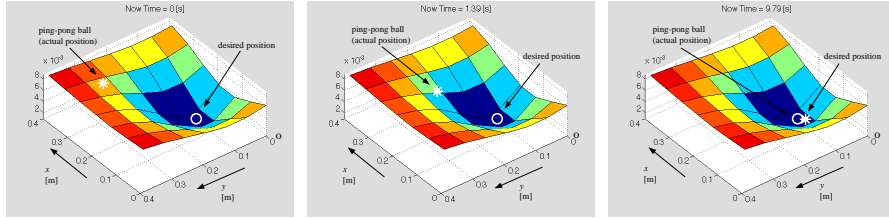
Fig. 14-a. Surface curve at 0.00 [s] (simulation) Fig. 14-b. Surface curve at 1.39 [s] (simulation) Fig. 14-c. Surface curve at 9.79 [s] (simulation)
