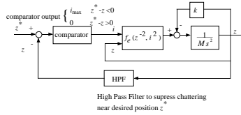
Fig. 8. Block diagram of solenoid plunger including variable structure controller and high pass filter.
