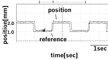
Fig. 10. Position response with variable structure controller. We can see a good agreement between the command and actual position.
