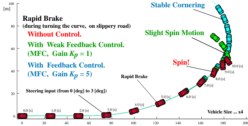
Fig. 10: Stabilizing effect with “controlled four wheels” is visualized with vehicle’s trajectory [6].
