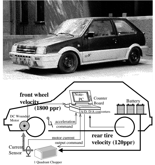
Fig. 7: “UOT Electric March-I”.
