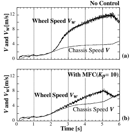
Fig. 9: Proposed controller changes the wheel dynamics to be insensitive to the road condition.
