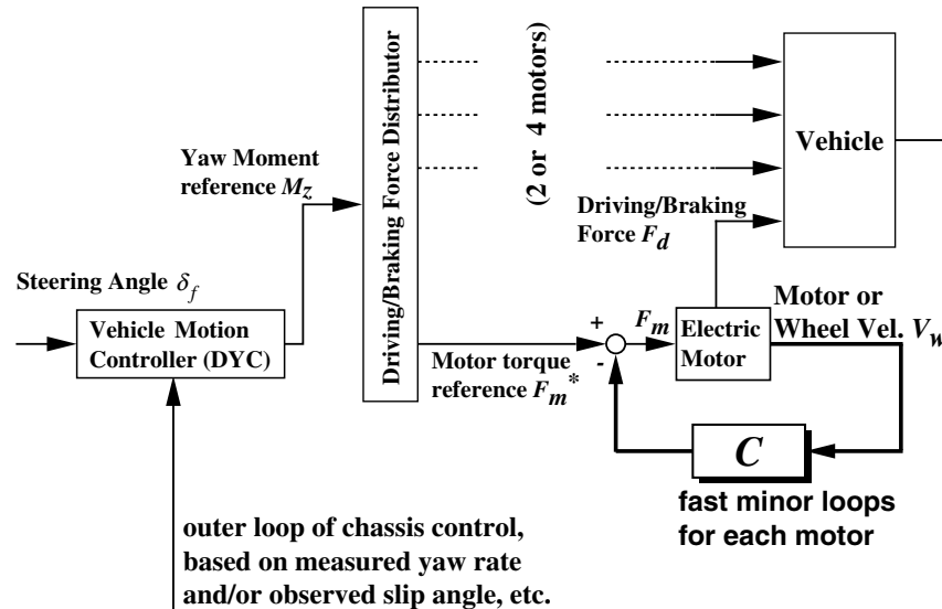
Fig. 15: Our idea for total system: chassis controller with fast minor loops.
