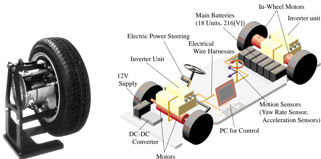
Fig. 1: In-wheel motor (left) and our new EV with four in-wheel motors. (right)
