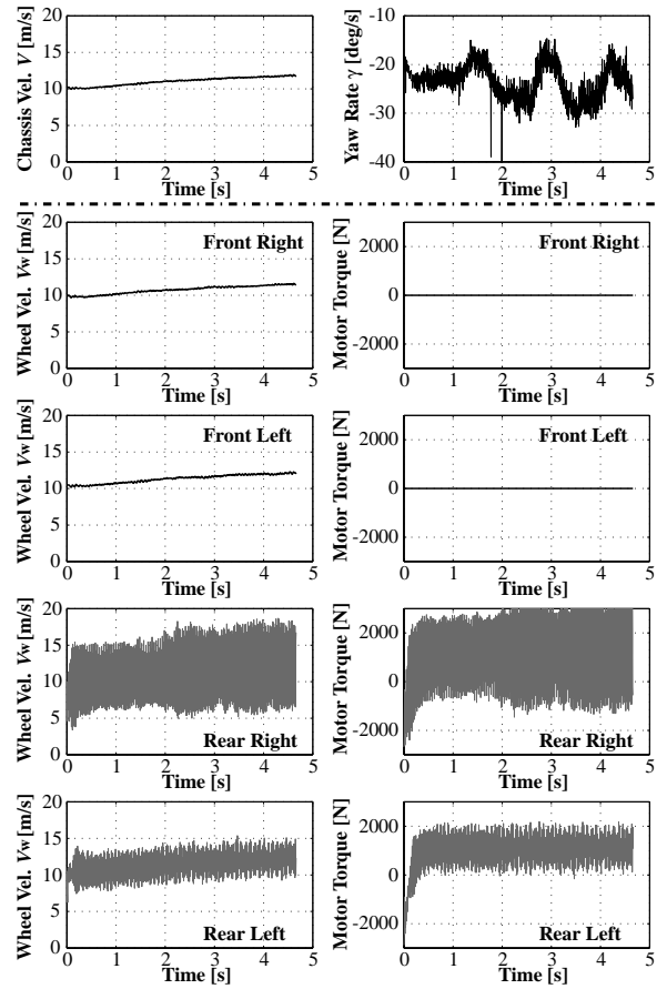
Fig. 13: Stabilizing effect of wheel velocity feedback. Proposed controller of Fig. [?] was applied on both rear wheels.
