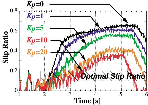
Fig. 8: Effect of wheel velocity control for skid prevention with \tau=0.1 [s] (Experimental results.) K_p^* of Eq. (16) is 4.52 for this vehicle.
