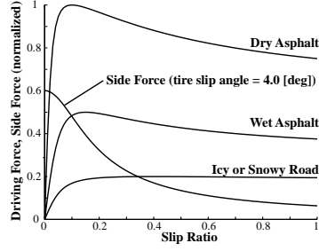
Fig. 3: One wheel model. Fig. 4: Typical \mu - \lambda curve.
