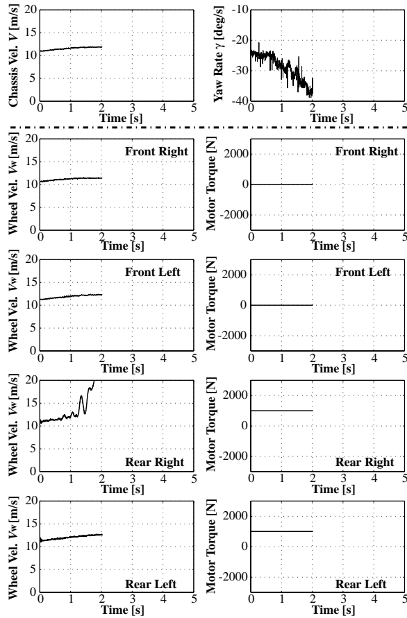
Fig. 12: Unstable turning with sudden acceleration torque on rear wheels. Vehicle made steady turning before torque inputs.
