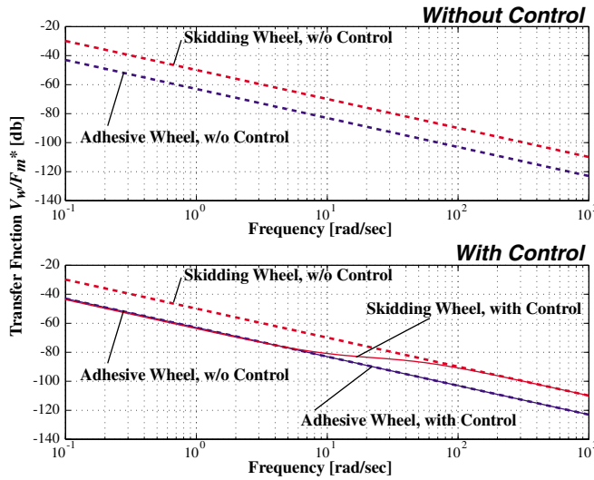
Fig. 6: Bode diagram of V_w/F_m^* .
