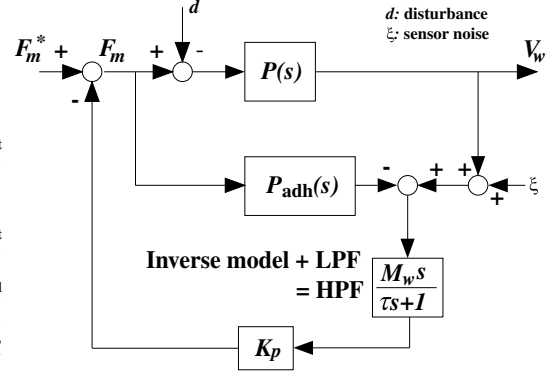
Fig. 5: Proposed feedback controller.
