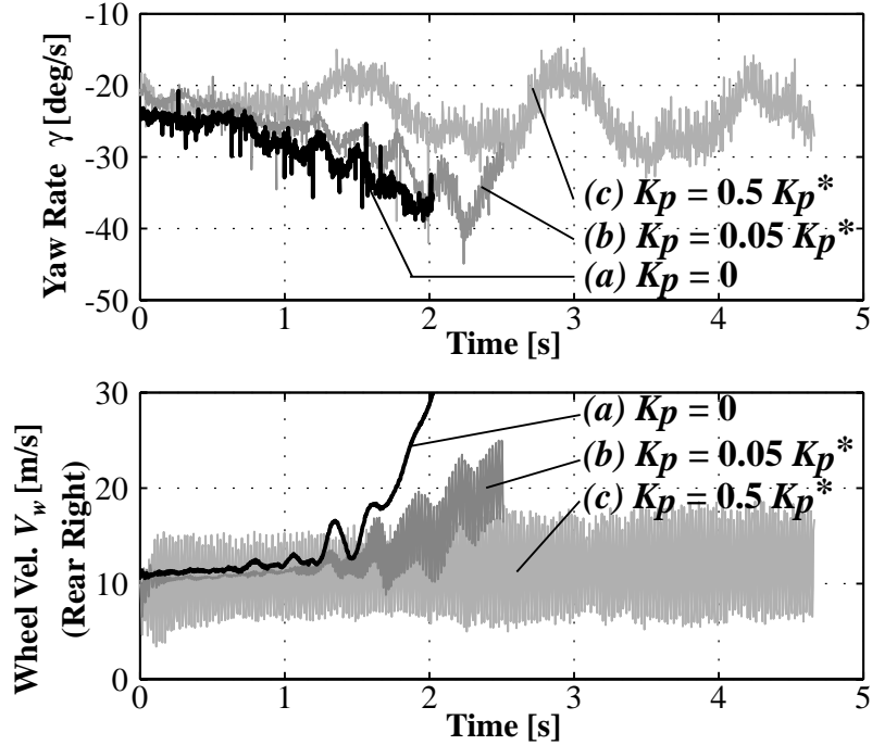
Fig. 14: Comparison of vehicle motion: (a) without feedback controller, (b) with weak feedback controller, (c) and adequate feedback controller. K_p^* of Eq. (16) is 45.2 for this vehicle. \tau in the controller was 0.1 [s].
