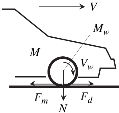
Figure 2: One wheel model.
