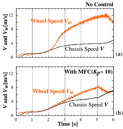
Figure 9: Wheel and chassis velocity with and without control.
