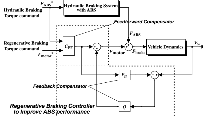
Figure 14: Block diagram of proposed controller.
