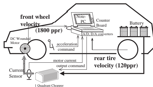
Figure 7: Our experimental vehicle, “UOT Electric March-I”.
