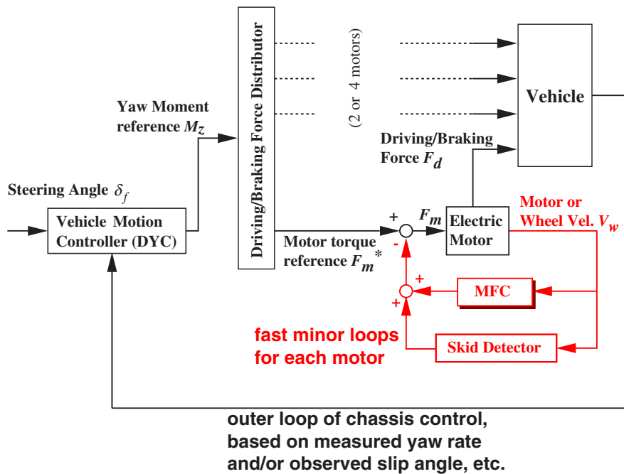
Figure 19: Our concept: minor-loop controller for each wheel.
