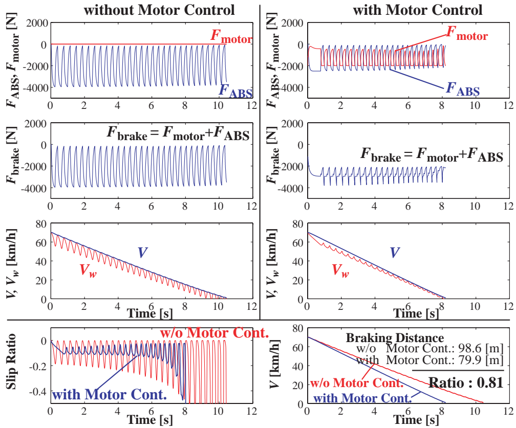
Figure 18: Simulation results with slippery road. ( F_{\text{motor}}^* = -1500 [N])
