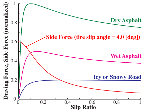
Figure 3: \mu - \lambda curve.
