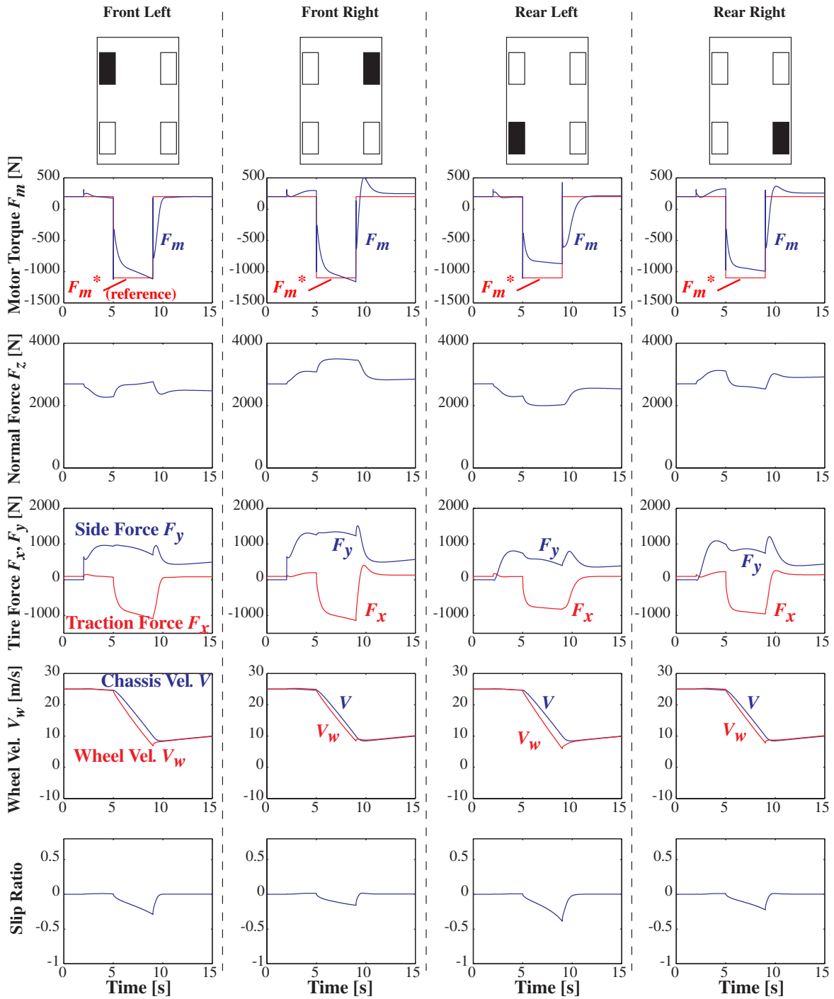
Figure 12: Simulation results of rapid braking on slippery road, during turning the curve with controlled four wheels. The driver's braking torque input is the same as Fig. 11, however, the vehicle is still stable.
