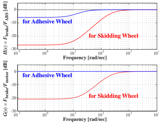
Figure 15: Bode diagram of H(s) , G(s) .
