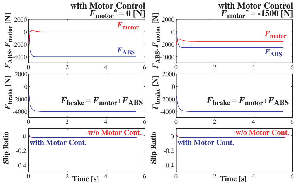
Figure 17: Simulation results with adhesive road.
