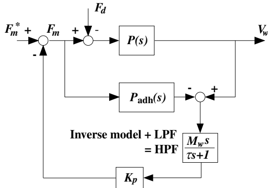
Figure 4: Block Diagram of wheel velocity controller.
