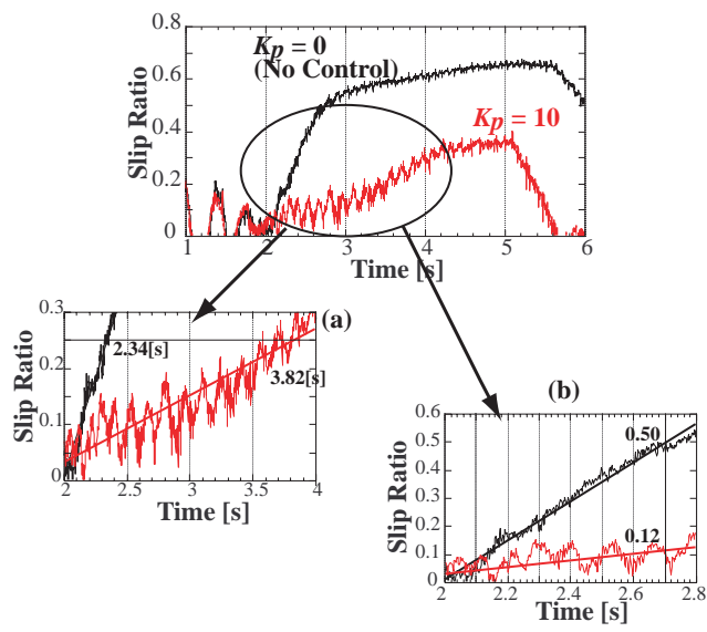
Figure 10: Effect of “slow” slip growth with proposed method.
