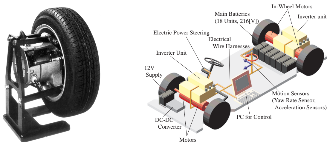
Figure 1: In-wheel motor and our new EV with four in-wheel motors.
