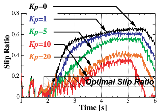
Figure 8: Effect of wheel velocity control for skid prevention with \tau=0.1 [s] (Left fig.: Experimental results / Right fig.: Simulation results)
