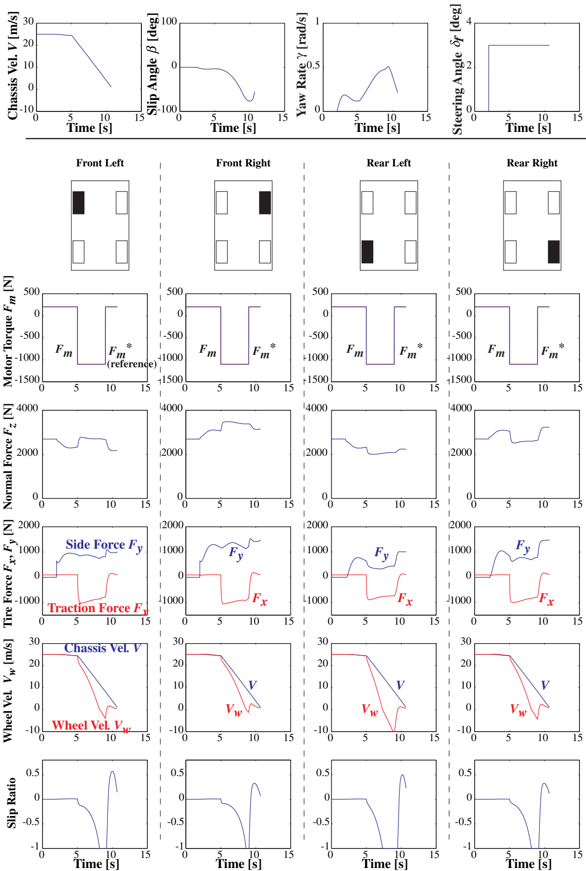
Figure 11: Example of unstable vehicle lateral motion. This is the simulation results of rapid braking on slippery road, during turning the curve.
