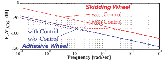
Figure 16: Bode diagram of H(s)P(s) .
