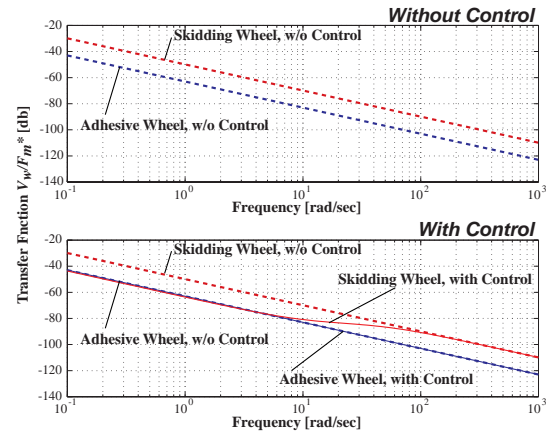
Figure 5: Bode diagram of V_w/F_m , with and without control.
