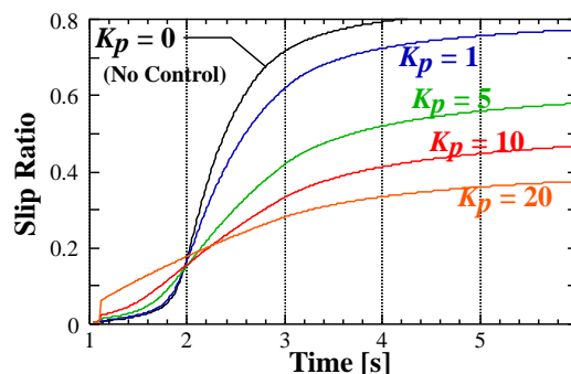
Figure 8: Effect of wheel velocity control for skid prevention with \tau=0.1 [s] (Left fig.: Experimental results / Right fig.: Simulation results)
