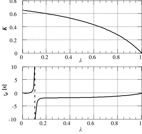
Fig. 3. Examples of K and \tau_a .
