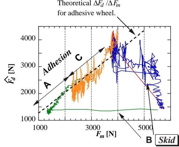
Fig. 9. F_m - F_d curve (experiment on dry asphalt).
