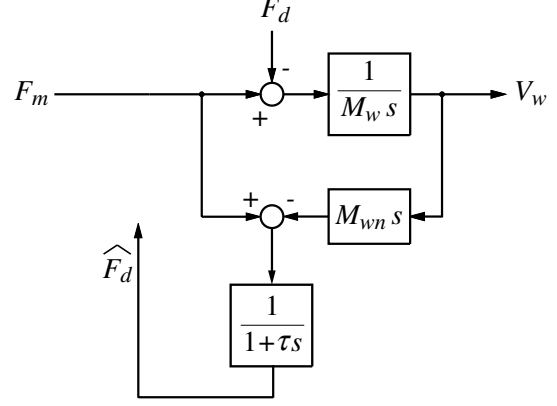
Fig. 4. Block Diagram of Disturbance Observer.
