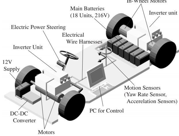
Fig. 18. Configuration of our new EV.
