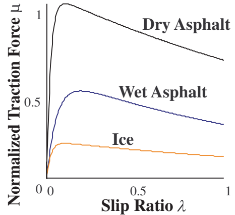
Fig. 2. Normalized traction force \mu plotted vs. slip ratio \lambda ( \mu - \lambda curve).
