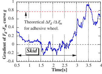
Fig. 12. g , the gradient of F_m-F_d curve (experiment on snowy road).
