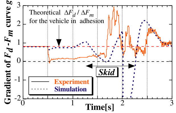
Fig. 15. g , the gradient of F_m-F_d curve (experiment on wet iron plate).
