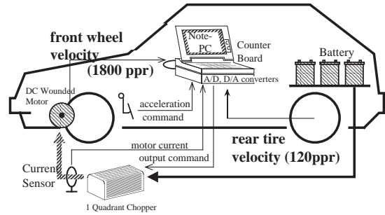
Fig. 6. Configuration of UOT Electric March I
