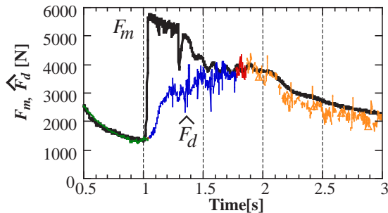
Fig. 8. Time response of F_m and F_d (experiment on dry asphalt).
