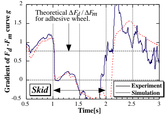
Fig. 10. g , the gradient of F_m - F_d curve (experiment on dry asphalt).
