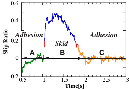
Fig. 7. Slip ratio (experiment on dry asphalt).
