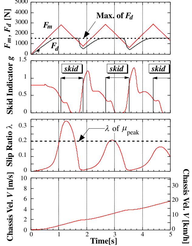
Fig. 17. Simulation results of skid prevention with proposed skid detector. \mu 's peak is at \lambda=0.2 .
