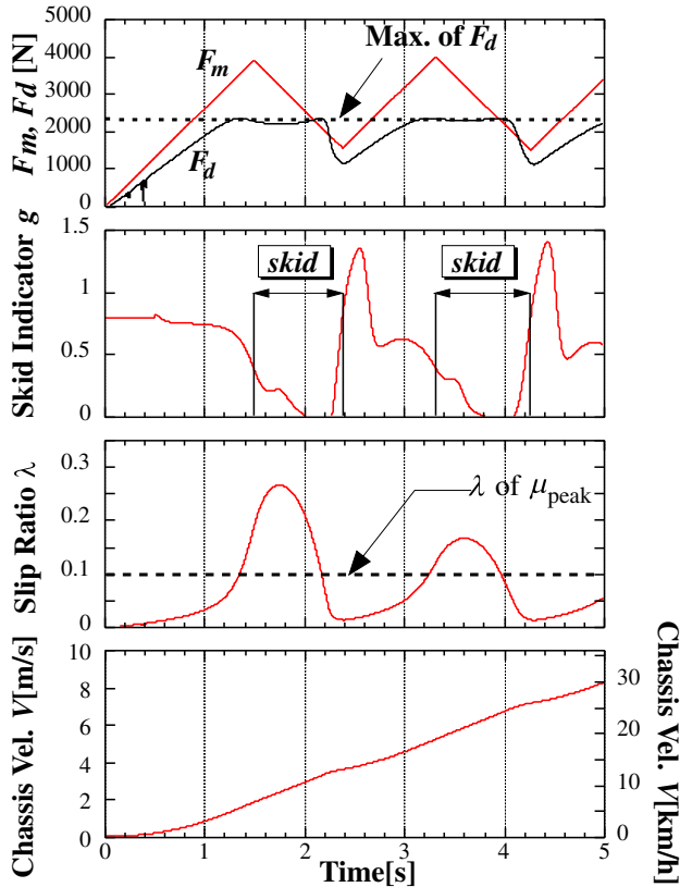
Fig. 16. Simulation results of skid prevention with proposed skid detector. \mu 's peak is at \lambda=0.1 .
