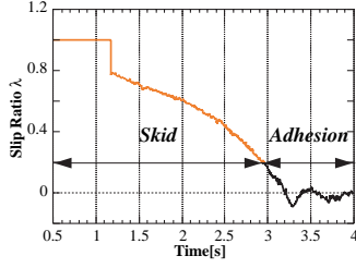
Fig. 11. Slip ratio (experiment on snowy road)
