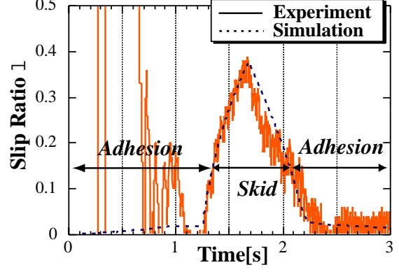
Fig. 14. Slip ratio (experiment on wet iron plate.)
