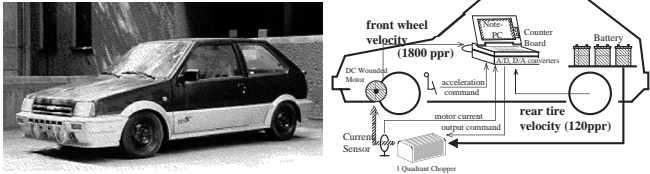
Fig. 6. Our experimental vehicle, "UOT Electric March-I".
