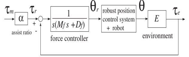
Fig. 9. Power assist control with conventional feedback controller.
