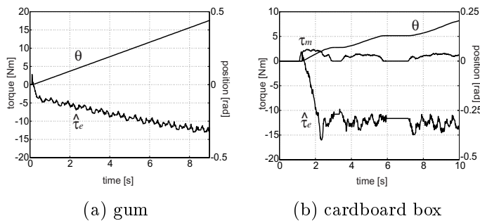
Fig. 4. Estimation of the environmental torque.
