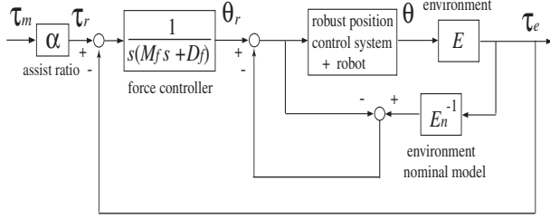
Fig. 12. Power assist control using environmental observer.
