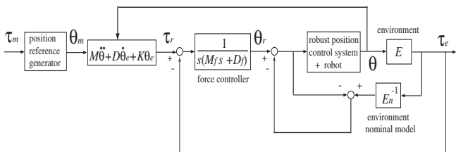
Fig. 17. Configuration of force control based method using impedance control.
