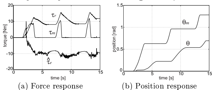
Fig. 18. Force control based method using impedance control (cardboard box).
