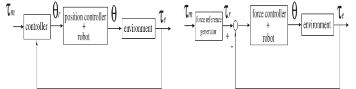
(a) Position control based method (b) Force control based method
