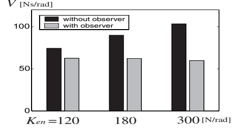
Fig. 14. Evaluation of the effectiveness of environmental observer.
