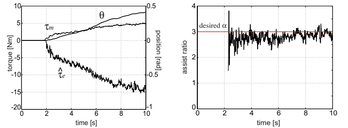
Fig. 8. Dual Impedance Control with stiffness impedance (cardboard box).
