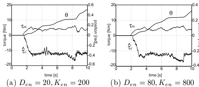
Fig. 16. Power assist control with environmental observer (cardboard box).
