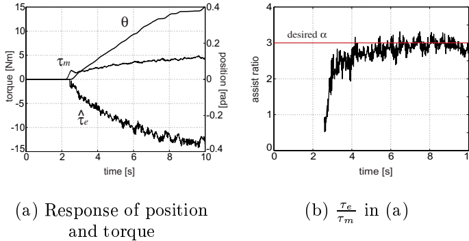
Fig. 13. Power assist control with environmental observer (gum).
