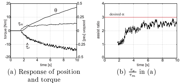
Fig. 6. Power assist experiment using Dual Impedance Control (gum).
