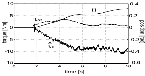
Fig. 8. Dual Impedance Control with stiffness impedance (cardboard box).
