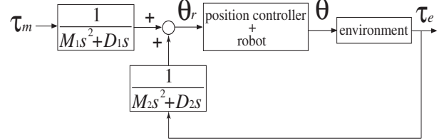
Fig. 5. Configuration of Dual Impedance Control.
