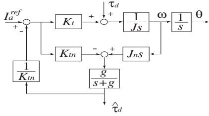
Fig. 3. Configuration of disturbance observer.
