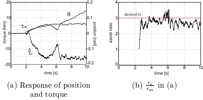
Fig. 7. Power assist experiment using Dual Impedance Control (cardboard box).
