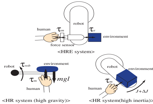
Fig. 1. Classification of power assist robot.
