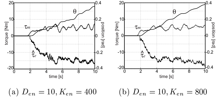
Fig. 15. Power assist control with environmental observer (cardboard box).
