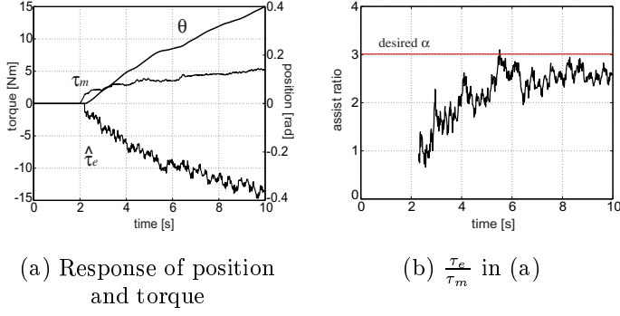
Fig. 11. Power assist control with conventional feedback controller (gum).
