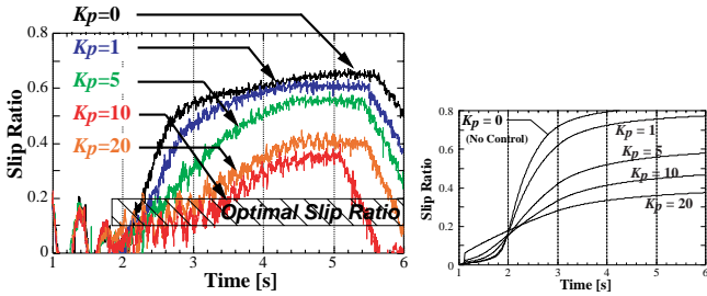
Fig. 7. MFC effect for skid prevention with \tau=0.1[s] (Left fig.: Experimental results / Right fig.: Simulation results)
