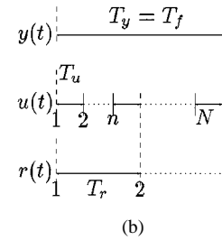
Fig. 2. Multirate sampling control. (a) Case 1 ( T_y \leq T_u ) (b) Case 2 ( T_y > T_u ).
