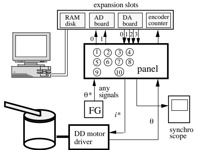
Fig. 1 Student experiment of Servo Control for all 3rd year students in undergraduate course.
