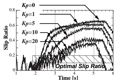
Fig. 2: Exp. results of wheel stabilization.
