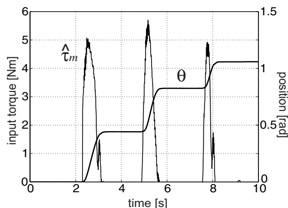
(b) M = 0.3, D = 6.0
