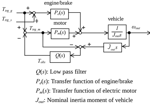
Figure 2: Calculation block of requested torque
