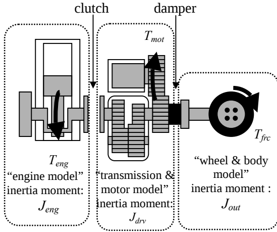
Figure 4: Vehicle physical model.
